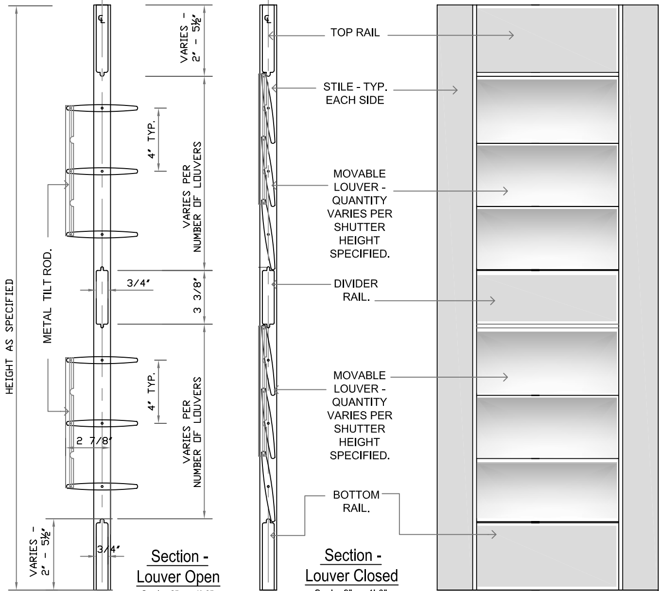
Front View Louver Closed Scale: 2" = 1'-0"
