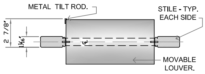
Plan View Louver Open Scale: 2" = 1'-0"
